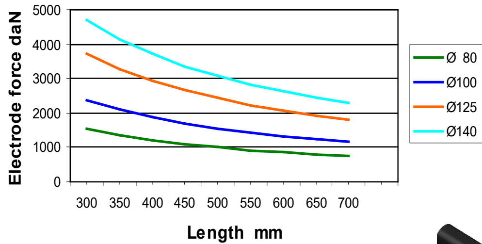
max. Electrode force at 5 bar
