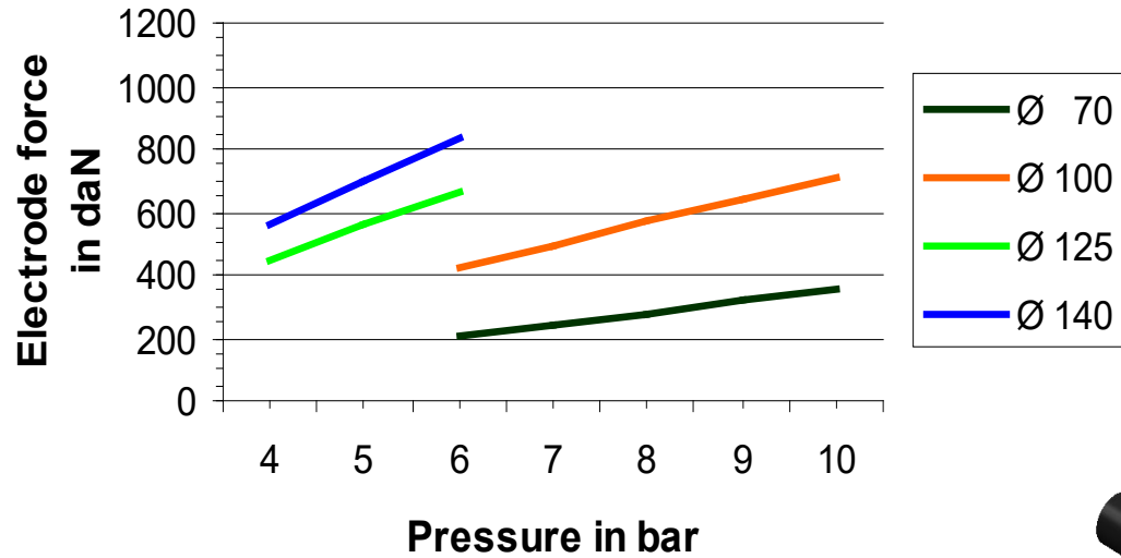
Electrode force
